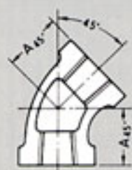
Fig 4 Elbows, Banded, 45°
