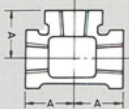
Fig 11A Tees, Banded, Equal
