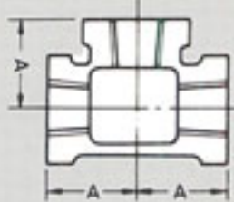
Fig 11A Tees, Banded, Equal
