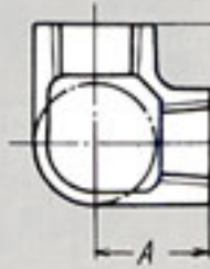
Fig 9 Side Outlet Elbows
