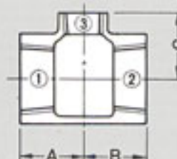
Fig 10B Tees, Plain, Reducing
