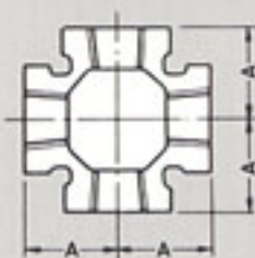
Fig 16 Crosses, Banded, Equal
