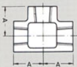
Fig 10A Tees, Plain, Equal
