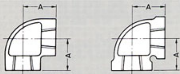
Fig 1A Elbows, Plain, Equal Fig 2A Elbows, Banded, Equal
