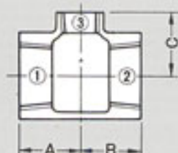
Fig 10B Tees, Plain, Reducing
