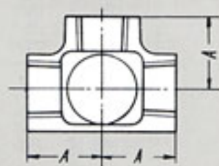
Fig 13 Side Outlet Tees
