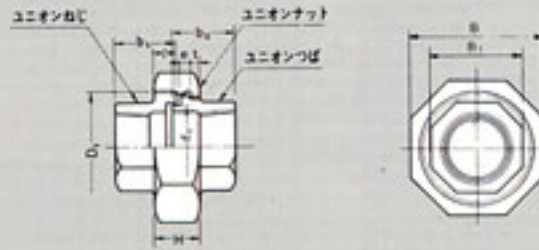
Fig 34A Unions, Standard, Flat Seat, without, Gasket
