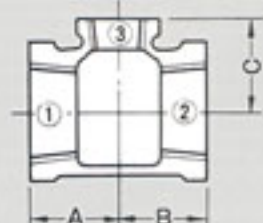
Fig 11B Tees, Banded, Reducing
